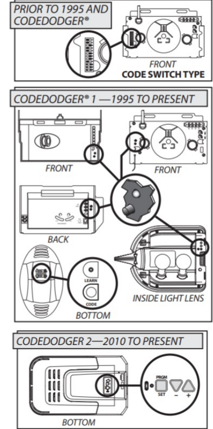
FIG. 1 POWERHEADS (for various models) Circle indicates location of Learn Code Button and LED.
